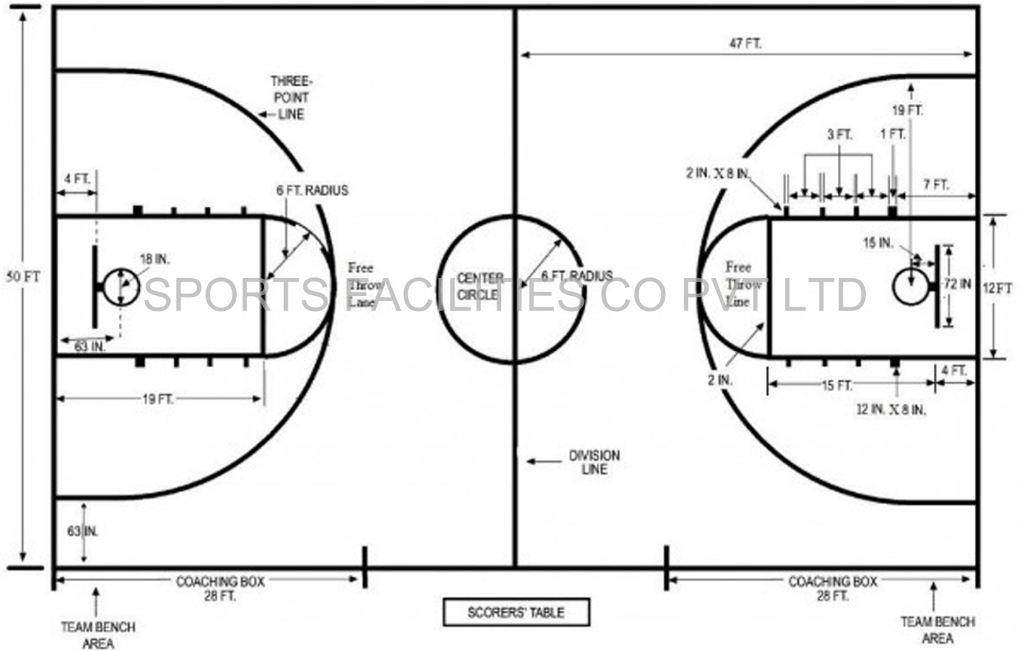
LAYOUT OF BASKETBALL COURT
